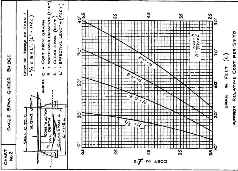
Fig. 254.—Cost of Single-span Girder Bridges.
